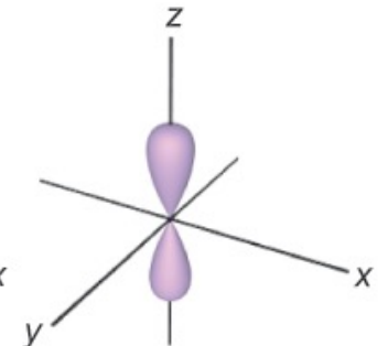
FIGURE 8.17 Shapes of p -orbitals
