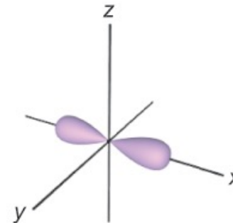
FIGURE 8.17 Shapes of p -orbitals
